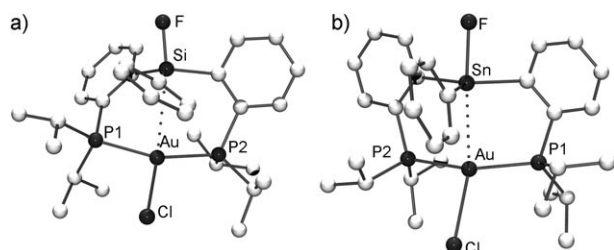
Figure 1. Molecular views of complexes 2 (a) and 4 (b) in the solid state (hydrogen atoms omitted for clarity). Selected bond lengths [Å] and angles ^\circ : 2 : P1–Au 2.323(2) , P2–Au 2.305(2) , Au–Cl 2.577(2) , Si–F 1.635(3) , Au–Si 3.090(2) ; P1–Au–P2 140.14(5) , Cl–Au–Si 141.54(4) , Au–Si–F 166.11(12) . 4 : P1–Au 2.334(2) , P2–Au 2.330(2) , Au–Cl 2.601(2) , Sn–F 2.018(3) , Au–Sn 2.891(2) ; P1–Au–P2 159.91(6) , Cl–Au–Sn 151.36(4) , Au–Sn–F 176.27(9) .
